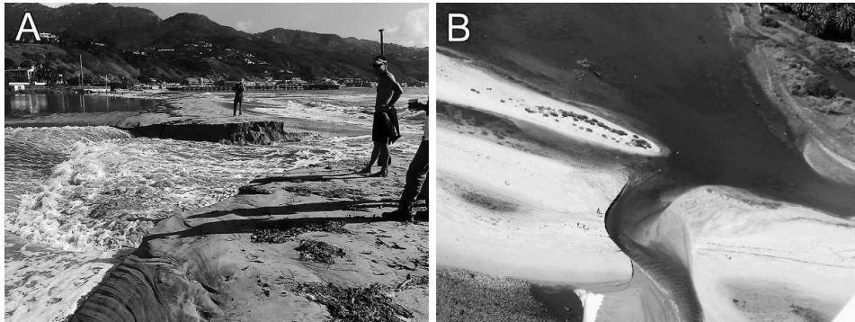
Fig. 2. Breach in the Malibu Lagoon sandbar, which was artificially created on October 7, 2010. A) Water coursing through the berm at 0947 h, shortly after the breach ruptured. B) Aerial view of the southeast portion of Malibu Lagoon on October 7, 2010 at 1315 h, showing a stream of lagoon water running through the breach, across the sandy beach, and onto the intertidal. A field of intertidal cobbles is visible at the lower left. (Photos courtesy H. Burdick, Los Angeles Waterkeeper).
